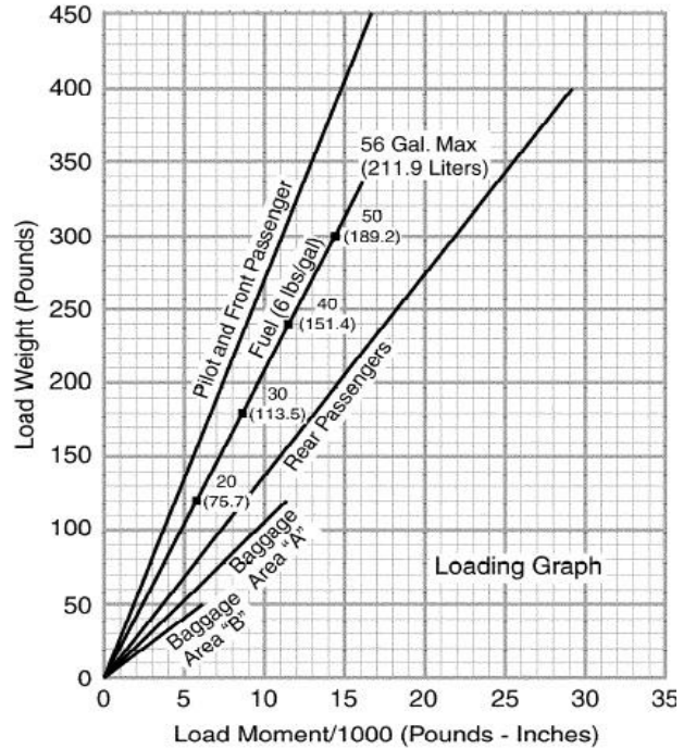
LOADING GRAPH
