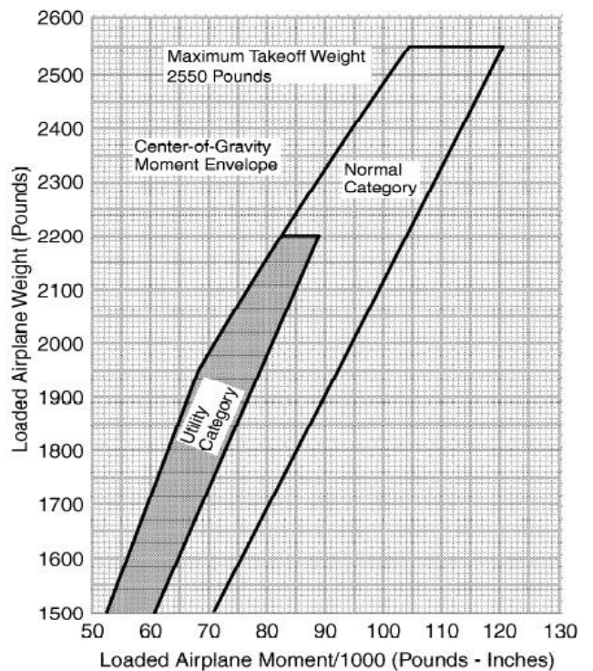
CENTER-OF-GRAVITY MOMENT ENVELOPE
